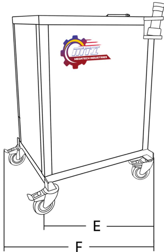
REAR VIEW
