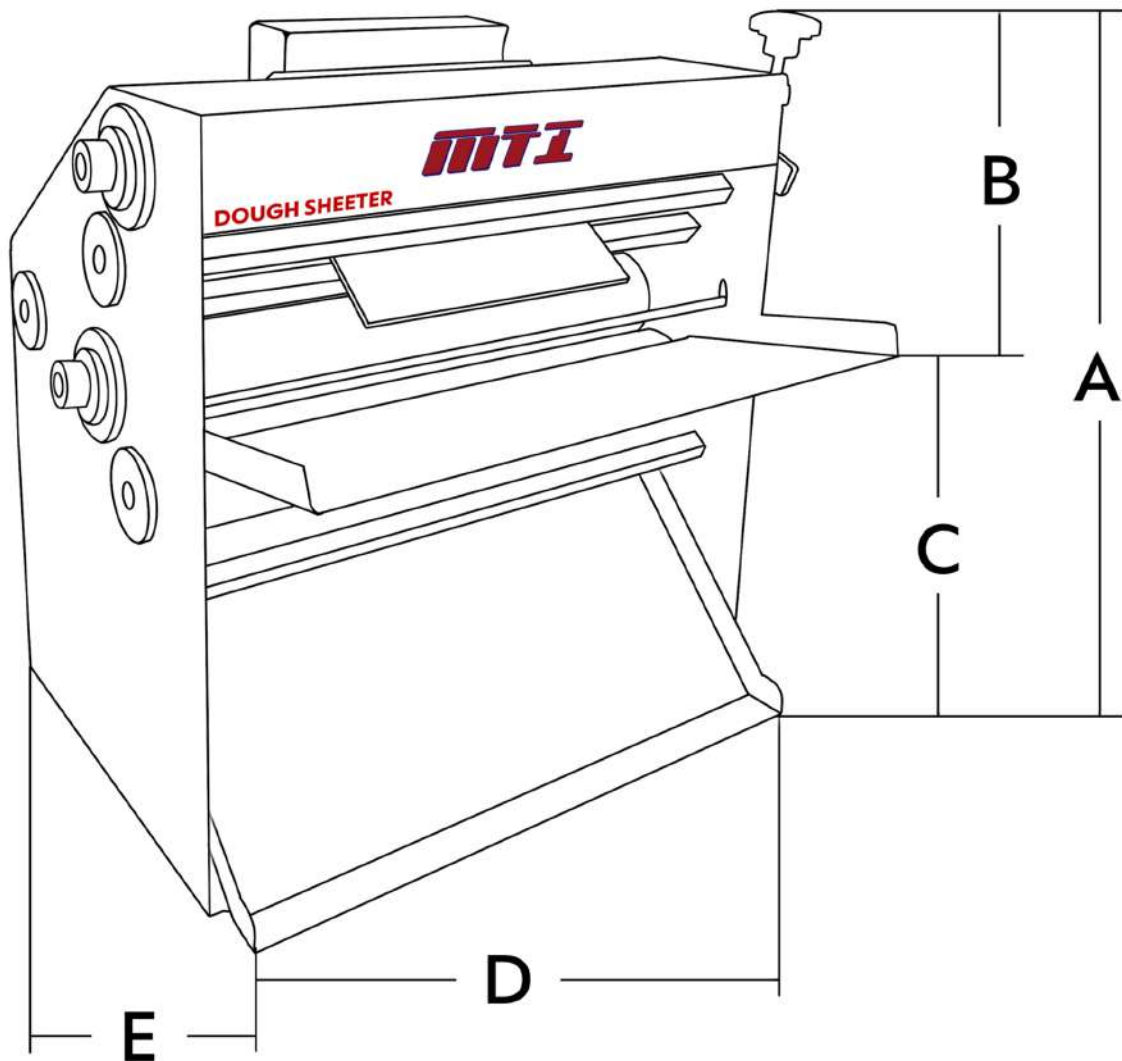
MEASUREMENTS - FRONT VIEW
