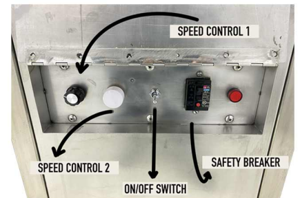
CONTROL PANNEL
