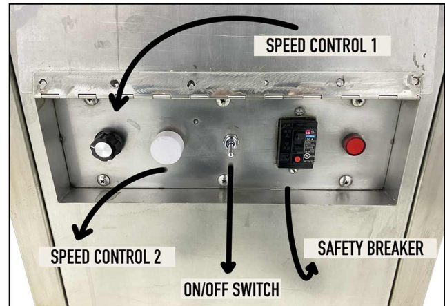
CONTROL PANNEL
